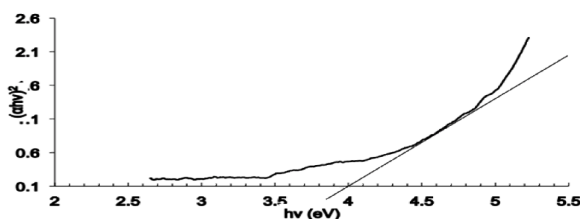
Fig. 5c. A plot of (\alpha hv)^2 versus hv for FTO annealed under N_2 at 573K.
